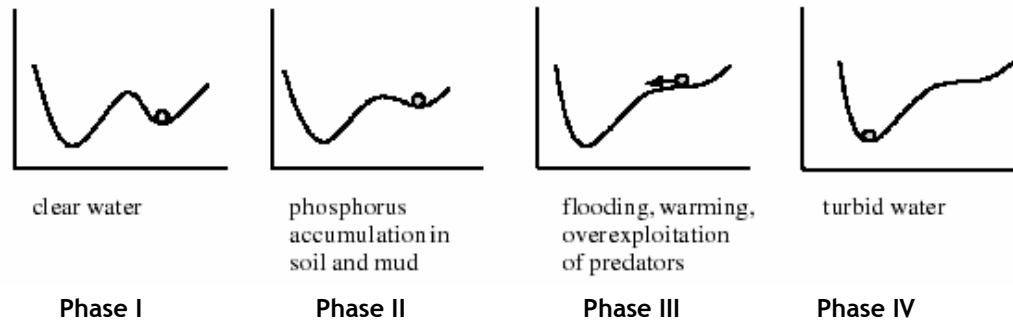
Figure 1. Resilience and Water Clarity (from Folke 2003)
